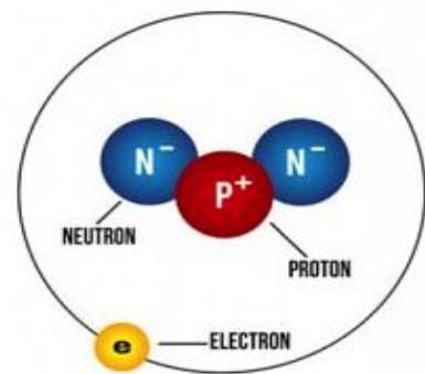
TRITIUM {}^3_1\text{H}
